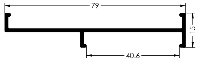
Ref. 6128 UNION DE CERCOS 73 Y PRACTICABLE 40
