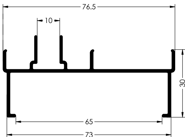
Ref. 6102 CERCO LATERAL
