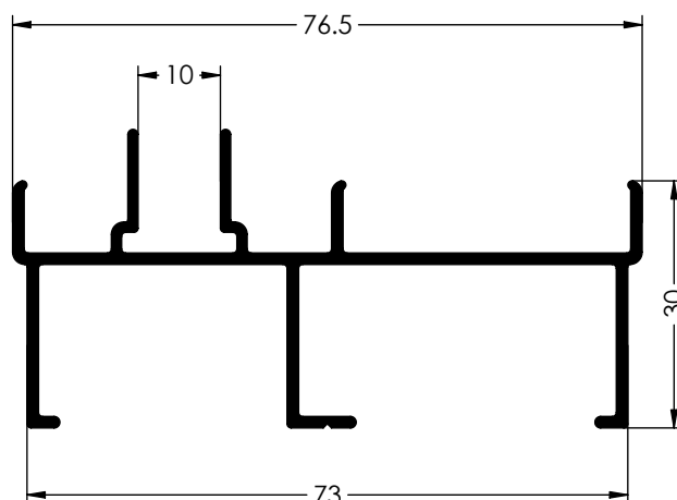
Ref. 6102A CERCO LATERAL
