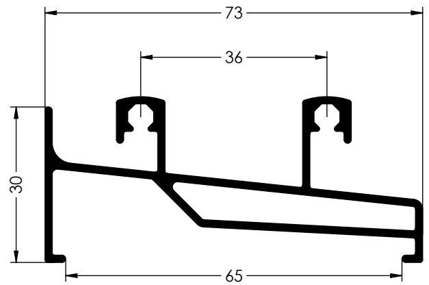
Ref. 6095 CERCO INFERIOR TUBULAR
