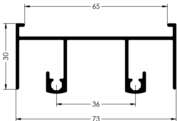
Ref. 6100 CERCO SUPERIOR
