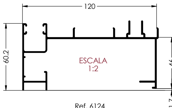
Ref. 6124 CERCOS LATERAL DCHO. CAJON MONOBLOCK
