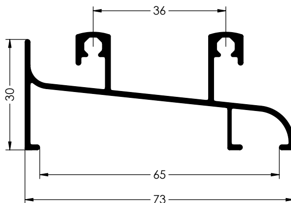
Ref. 6101 CERCO INFERIOR
