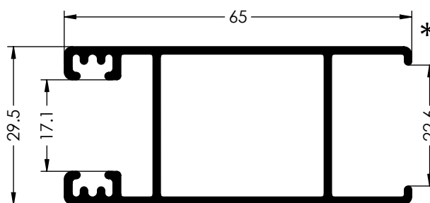
Ref. 6135 HOJA LATERAL CLIMALIT
