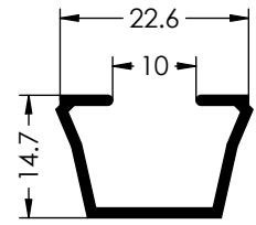
Ref. 6106 COMPL. CRISTAL MONOLIT.
