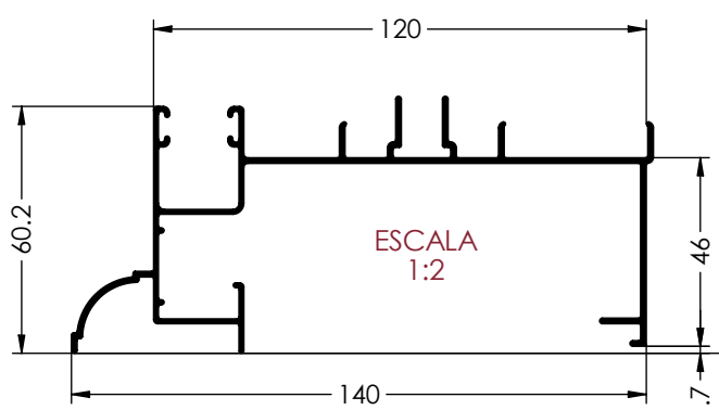
Ref. 6112 CERCOS LATERAL IZQ. CAJON MONOBLOCK
