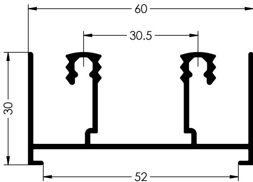
Ref. 6050 CERCOS SUPERIORES
