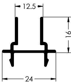
Ref. 6063 COMPLEMENTO 4 HOJAS
