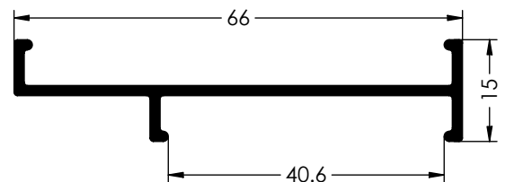
Ref. 3386 UNION CERCOS LATERAL CON PRACTICABLE
