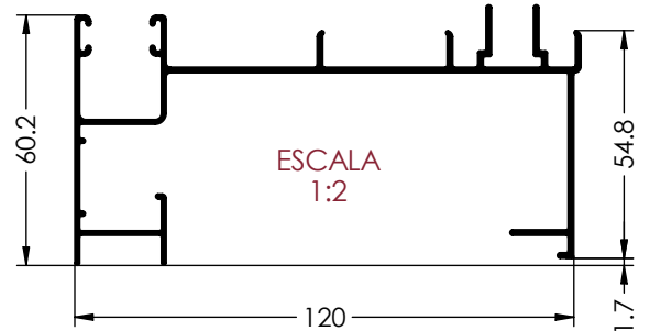
Ref. 6130 CERCOS LATERAL DERECHO (MONOBLOCK)
