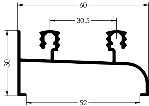
Ref. 6051 CERCOS INFERIORES
