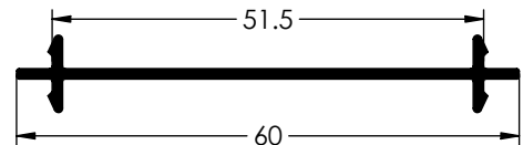
Ref. 6068 UNION CERCOS
