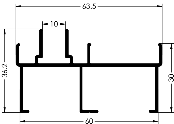
Ref. 6072 CERCOS LATERALES
