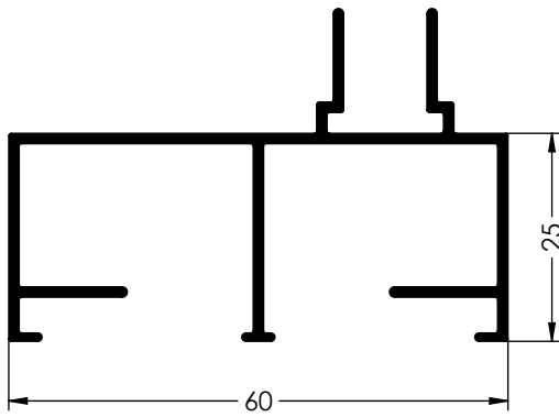
Ref. 6045 CERCOS LATERAL
